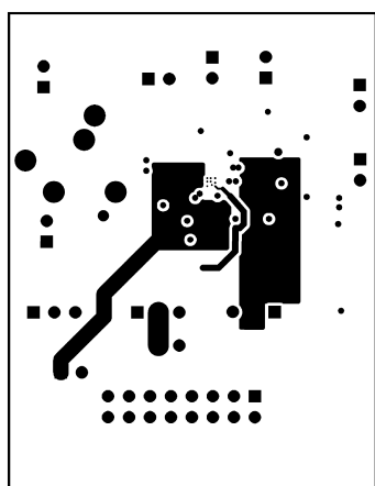
Figure 47. Internal Layer 2
