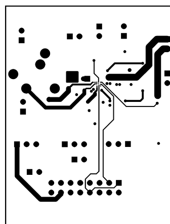
Figure 48. Bottom Layer
