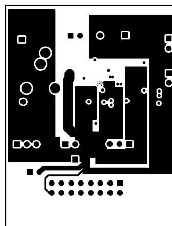
Figure 46. Internal Layer 1
