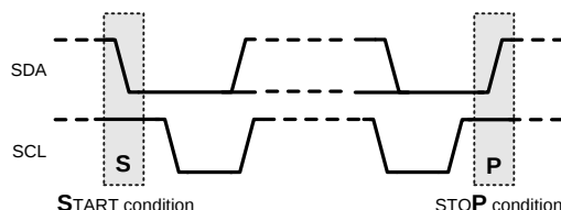
Figure 40. Start and Stop Diagram
