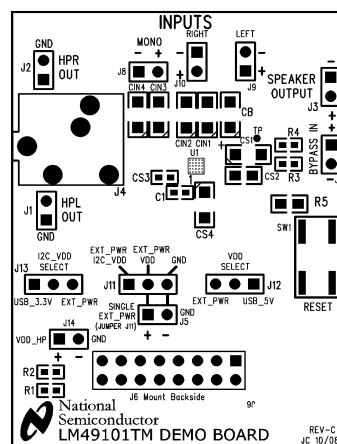
Figure 44. Silk Screen
