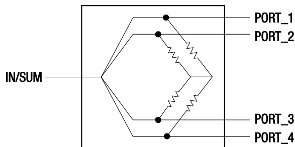
Figure 1. PD4W18-59LF Block Diagram
