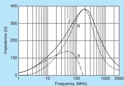
BLM21AG331SN1
