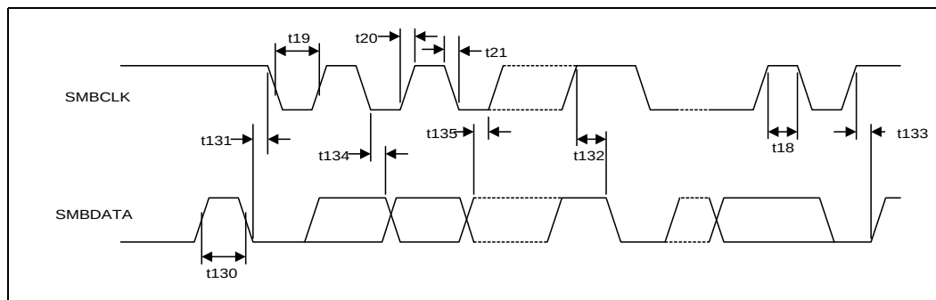
Figure 8-21. SMBus Timeout
