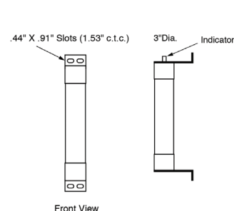
Bolt-In Mount "BI"
