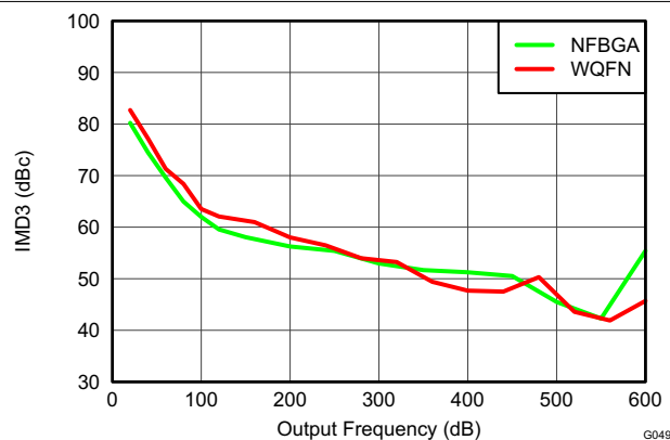
Figure 5-48. IMD3 vs Output Frequency
