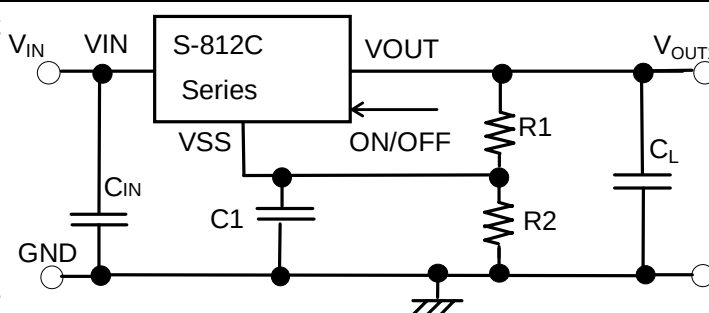
Figure 13 Voltage Adjustment Circuit
