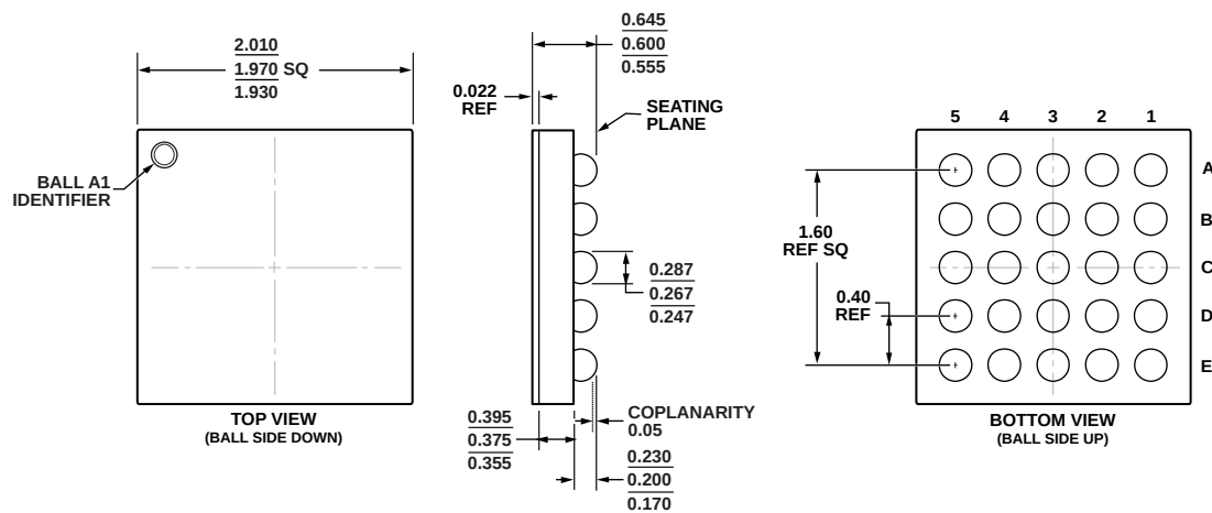
Figure 22. 25-Ball Wafer Level Chip Scale Package [WLCSP]
