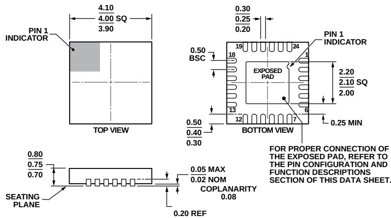
Figure 21. 24-Lead Lead Frame Chip Scale Package [LFCSP_WQ]
