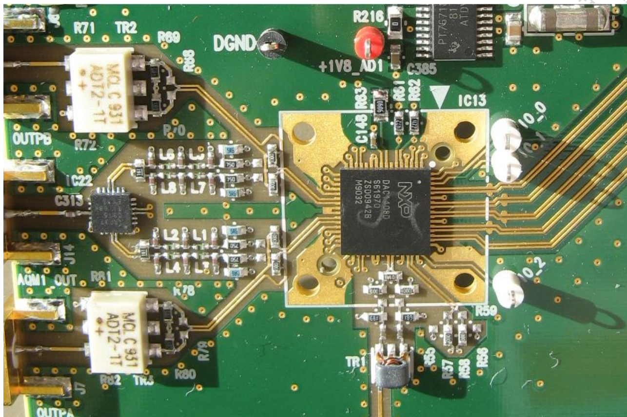
(1) NXP serial DAC device (9x9mm package)
