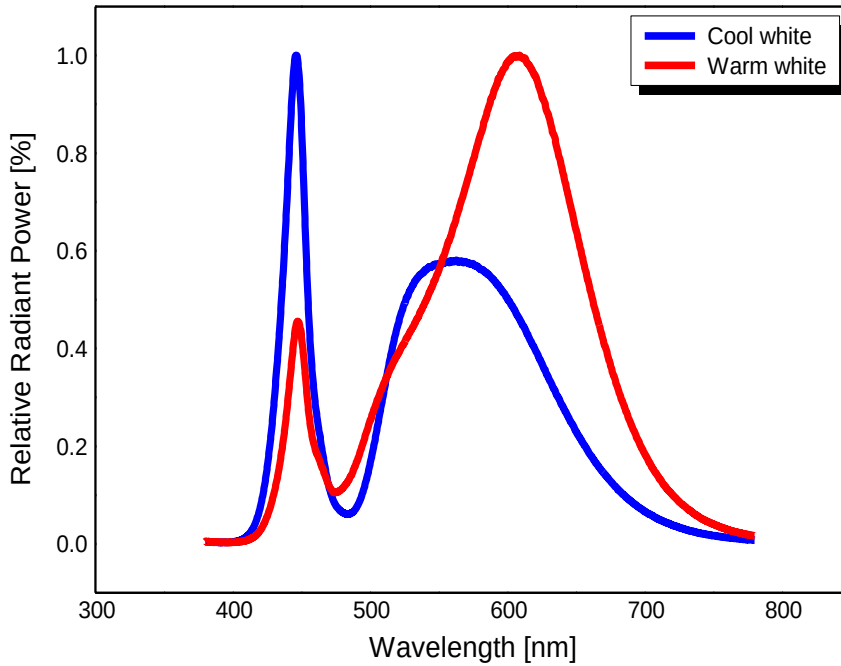
Fig 1. Color Spectrum, T_a = 25^{\circ}\text{C} , I_F = 180\text{mA} , RH30%
