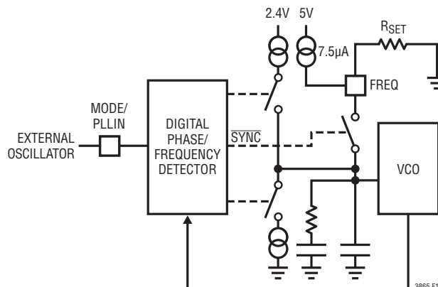
Figure 11. Phase-Locked Loop Block Diagram
