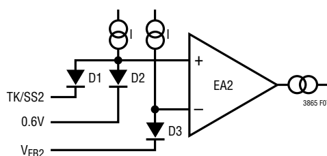
Figure 7. Equivalent Input Circuit of Error Amplifier
