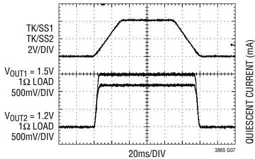
Tracking Up and Down with External Ramp (Forced Continuous Mode)
