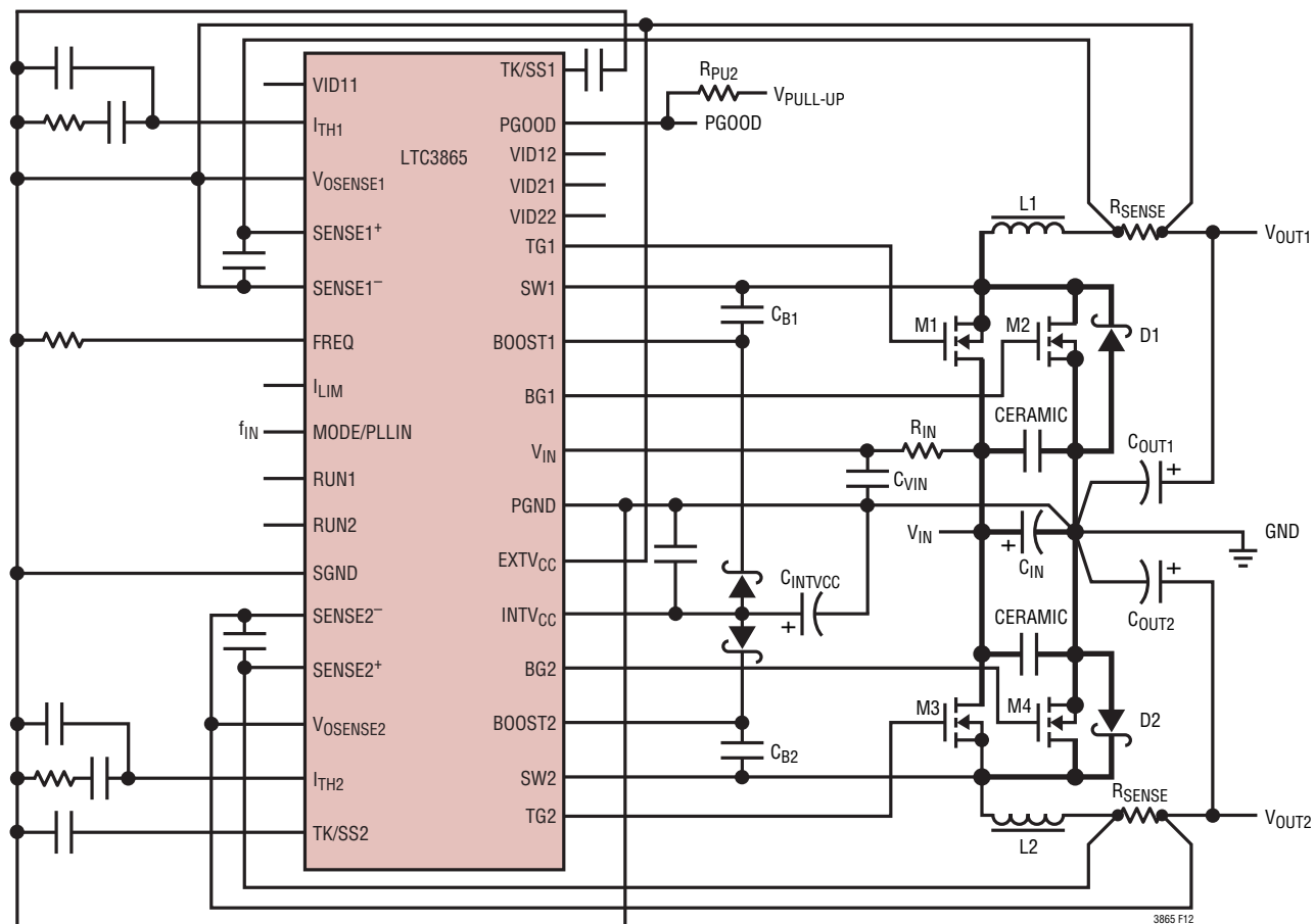
Figure 12. Recommended Printed Circuit Layout Diagram
