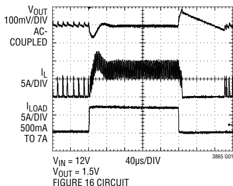
Load Step (Burst Mode Operation)
