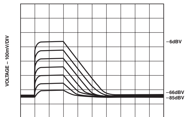
TPC 10. Large Signal Transient Response
