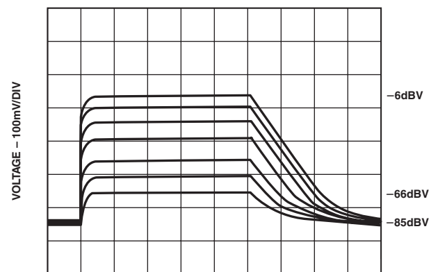
TPC 11. RMS Level Detector Performance with C_{AVG} = 22 \mu F
