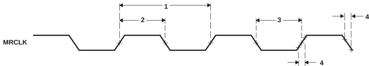
Figure 7-48. MRCLK Timing
