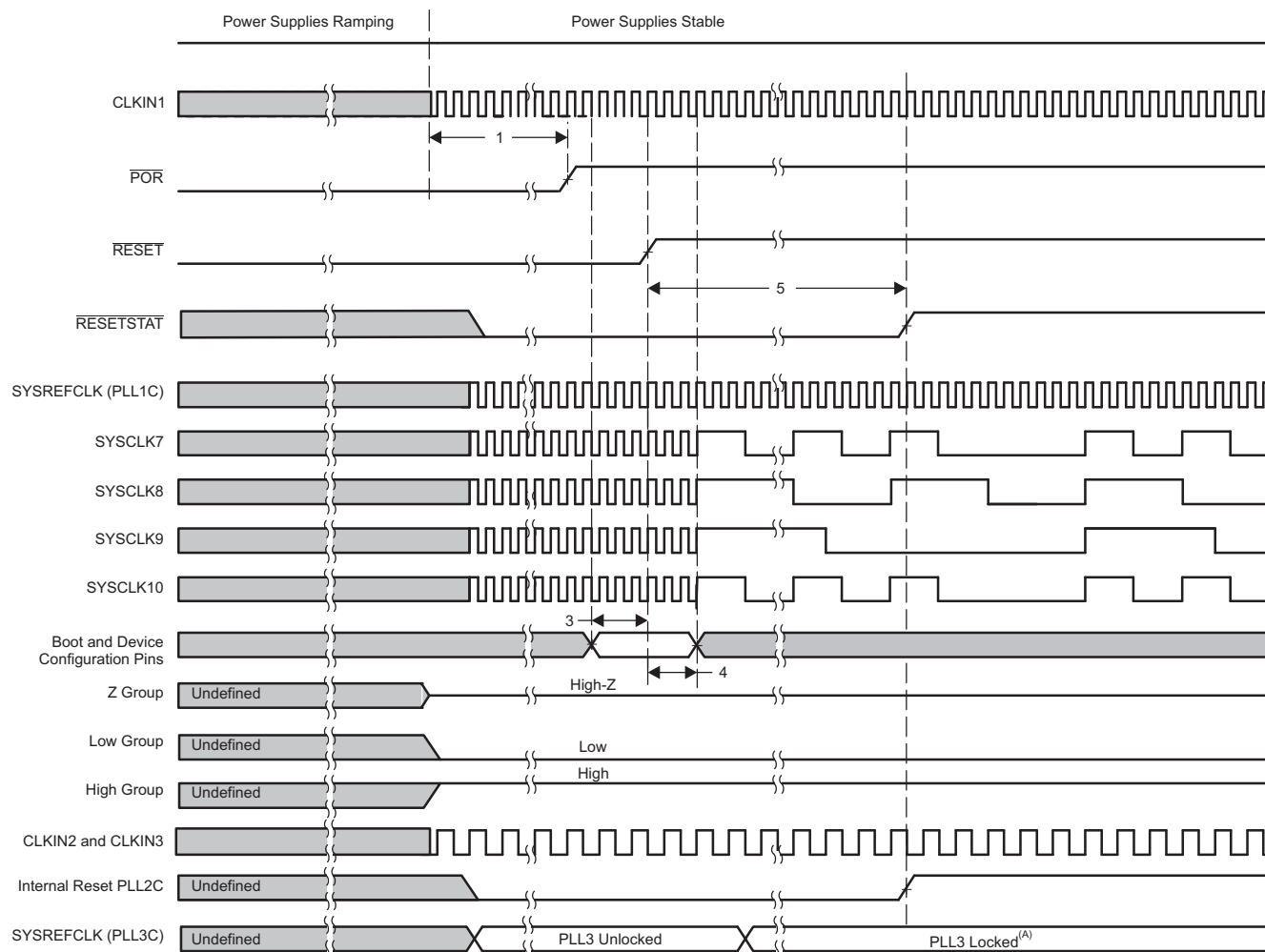
Figure 7-9. Power-Up Timing
