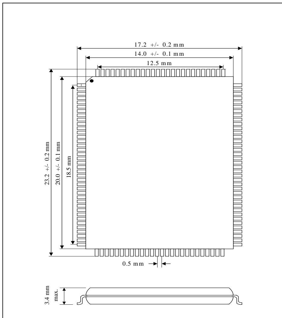
Figure 25: 128-pin PQFP Package Outline Drawing
