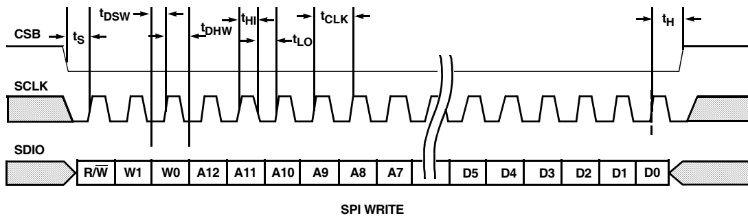
FIGURE 37. SPI WRITE
