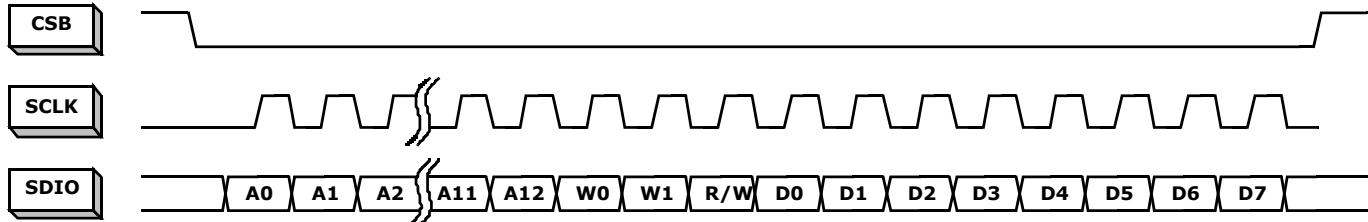
FIGURE 36. LSB-FIRST ADDRESSING
