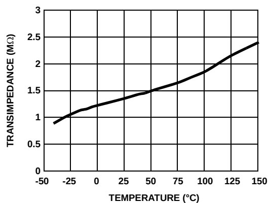
FIGURE 22. TRANSIMPEDANCE vs TEMPERATURE
