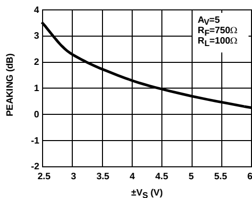
FIGURE 6. DIFFERENTIAL PEAKING vs SUPPLY VOLTAGE
