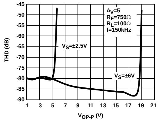
FIGURE 8. DIFFERENTIAL TOTAL HARMONIC DISTORTION vs DIFFERENTIAL OUTPUT VOLTAGE
