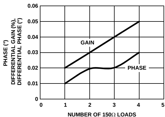
FIGURE 15. DIFFERENTIAL GAIN AND DIFFERENTIAL PHASE
