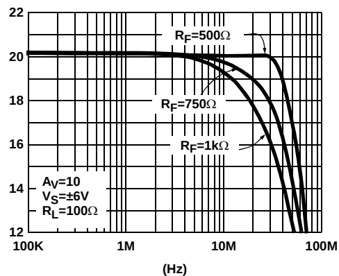
FIGURE 24. DIFFERENTIAL FREQUENCY RESPONSE vs R_F
