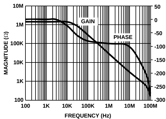
FIGURE 14. TRANSIMPEDANCE (ROL) vs FREQUENCY
