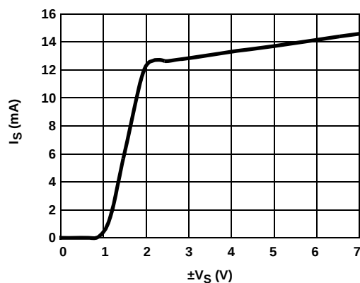
FIGURE 20. SUPPLY CURRENT vs SUPPLY VOLTAGE
