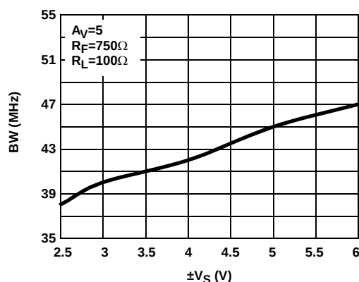
FIGURE 4. DIFFERENTIAL BANDWIDTH vs SUPPLY VOLTAGE
