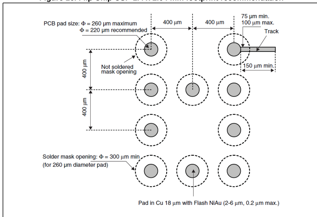
Figure 16. Flip Chip CSP 1.4 x 2.04 mm footprint recommendation
