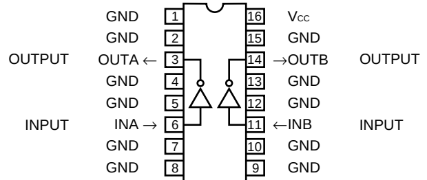
M66700WP Outline 16P4
