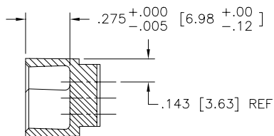
SECTION X-X
