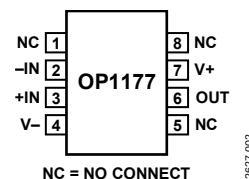
Figure 2. 8-Lead SOIC_N (R-Suffix)
