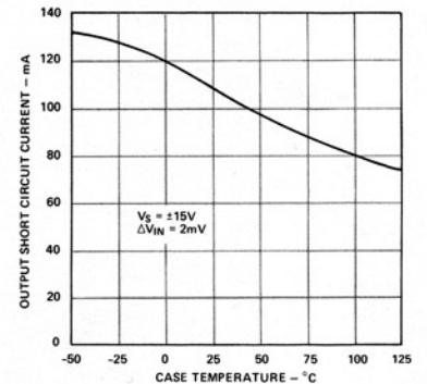
Figure 12. I_{SC} vs. Temperature
