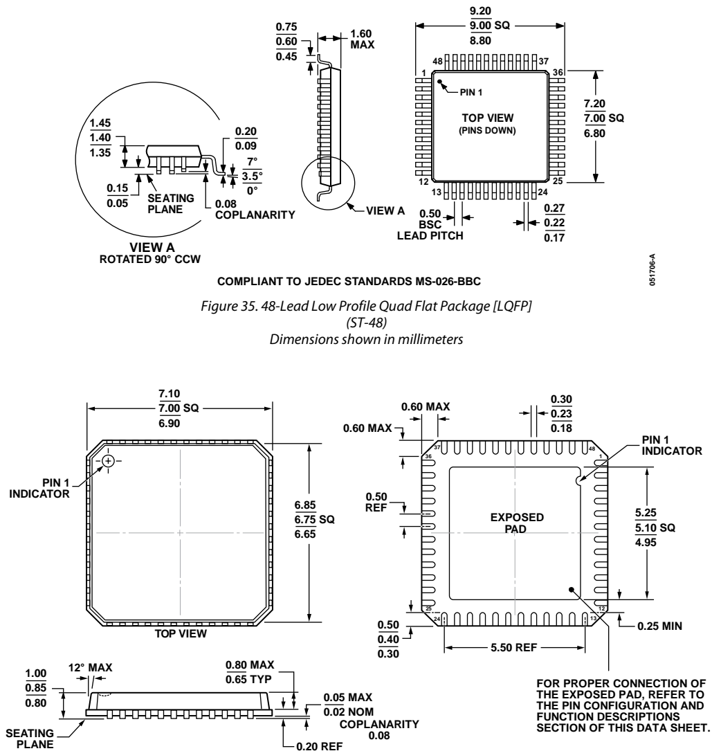
Figure 36. 48-Lead Lead Frame Chip Scale Package [LFCSP_VQ] 7 mm × 7 mm Body, Very Thin Quad (CP-48-1) Dimensions shown in millimeters
