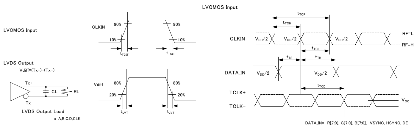
Figure-3 LVCMOS Input AC Timing Diagrams
