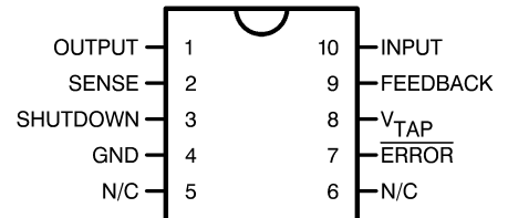
10-Lead Ceramic Surface-Mount Package (WG)
