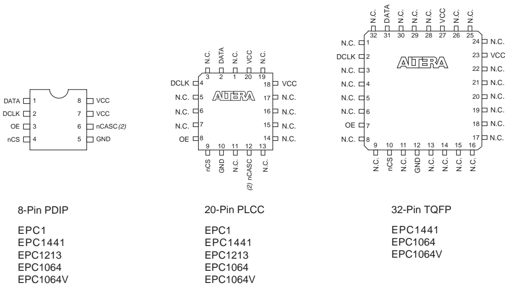
Figure 5–6. EPC1, EPC1441, EPC1213, EPC1064 & EPC1064V Package Pin-Out Diagrams Note (1)
