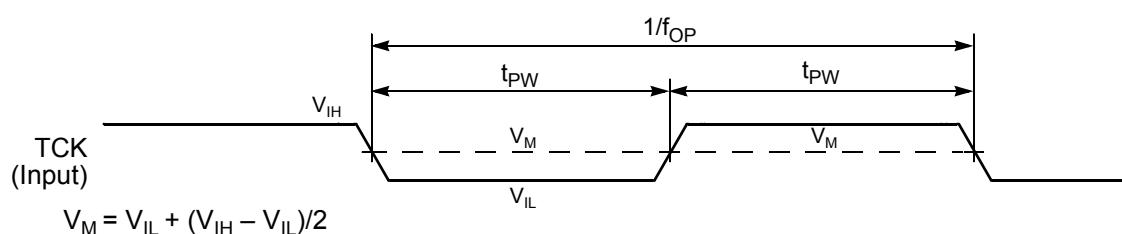
Figure 10-16 Test Clock Input Timing Diagram
