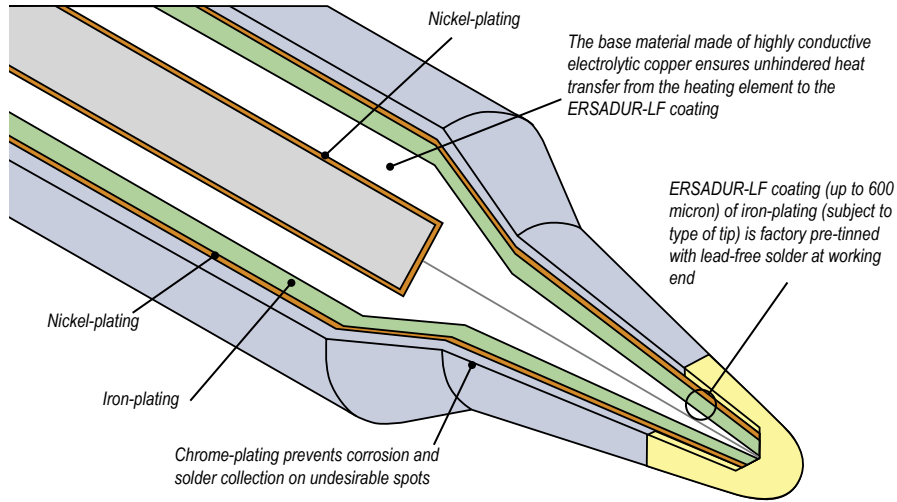
Cross-section of an ERSADUR soldering tip, non-scale representation
