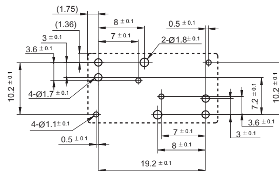
Twin relay
