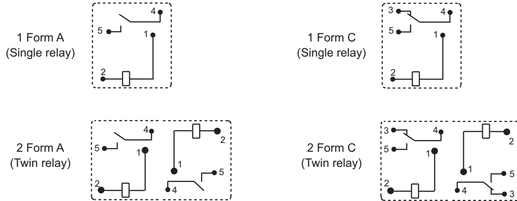
PCB Layout (Bottom view)
