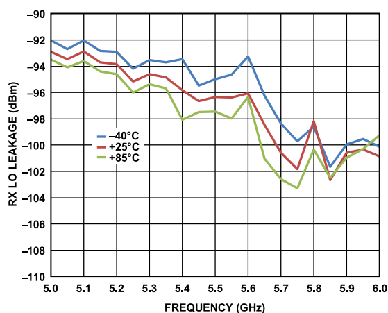
Figure 61. RX Local Oscillator (LO) Leakage vs. Frequency
