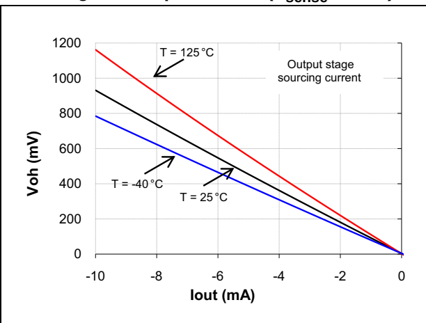
Figure 11. Output stage high-state saturation voltage vs. output current ( V_{\text{sense}} = +1\text{ V} )
