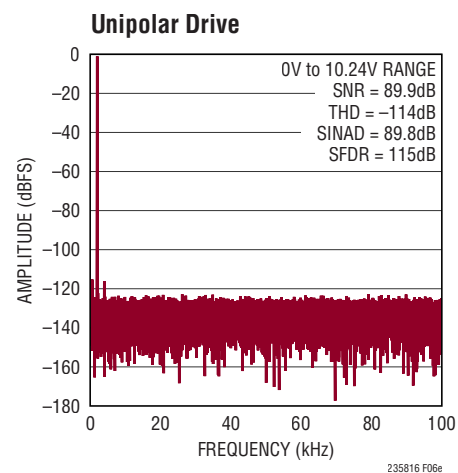
Figure 6e. IN^+ = -1\text{dBFS} 2kHz Unipolar Sine, IN^- = 0\text{V} , 32k Point FFT, f_{\text{SAMPL}} = 200\text{ksps} . Circuit Shown in Figure 6a
