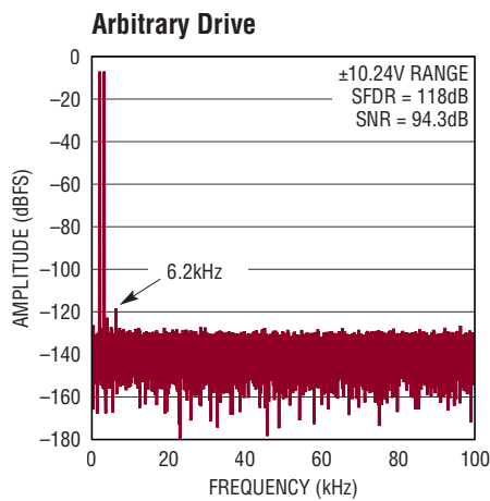
Figure 6b. Two-Tone Test. IN^+ = -7\text{dBFS} 2kHz Sine, IN^- = -7\text{dBFS} 3.1kHz Sine, 32k Point FFT, f_{\text{SAMPL}} = 200\text{ksps} . Circuit Shown in Figure 6a
