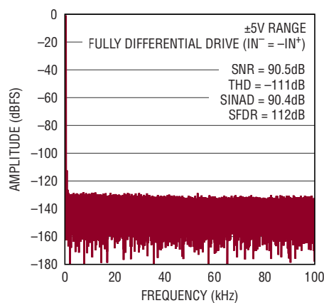
Figure 7c. IN^+/IN^- = 450\text{mV} 200Hz Fully Differential Sine, 0\text{V} \leq V_{CM} \leq 24\text{V} , 32k Point FFT, f_{SAMPL} = 200\text{ksps} . Circuit Shown in Figure 7a
