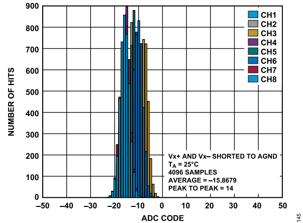
Figure 54. Histogram of Codes, ±20 V Differential Range Low Bandwidth Mode
