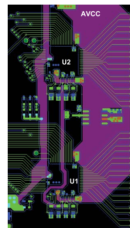
Figure 126. Layout for Multiple AD7606C-18 Devices—Top Layer and Supply Plane Layer
