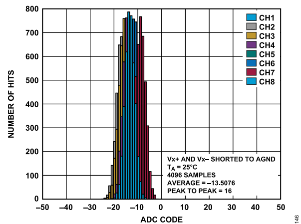
Figure 55. Histogram of Codes, ±10 V Single-Ended Range Low Bandwidth Mode
