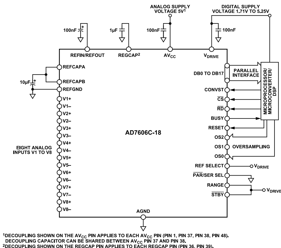
Figure 122. AD7606C-18 Typical Connection Diagram, Hardware Mode
