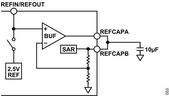
Figure 84. Reference Circuitry
