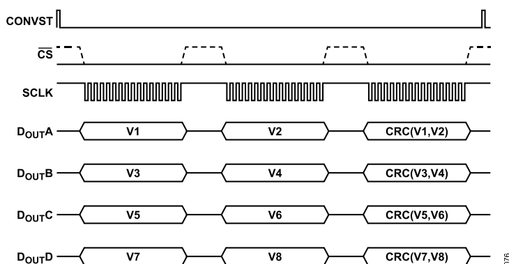
Figure 116. Serial Interface ADC Reading with CRC On, Four D OUT x Lines
