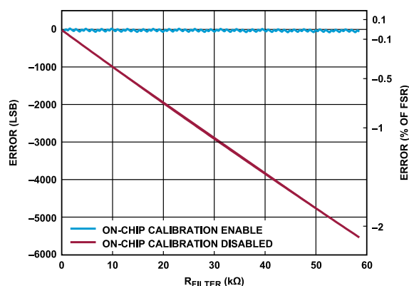
Figure 94. System Gain Calibration with and Without Calibration, \pm 10 V Single-Ended Range
