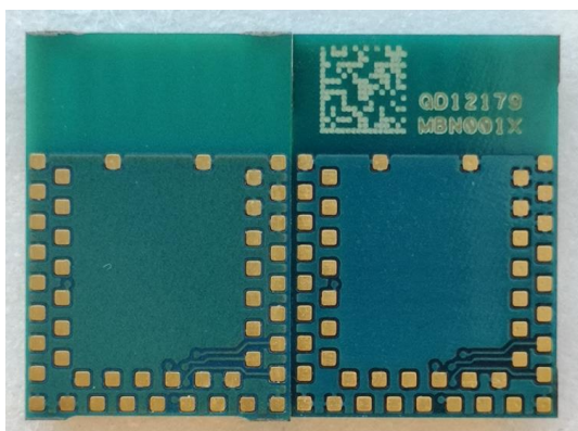
Figure 7: BMD-360-A-R-20 data matrix and marking example on PCB bottom side
