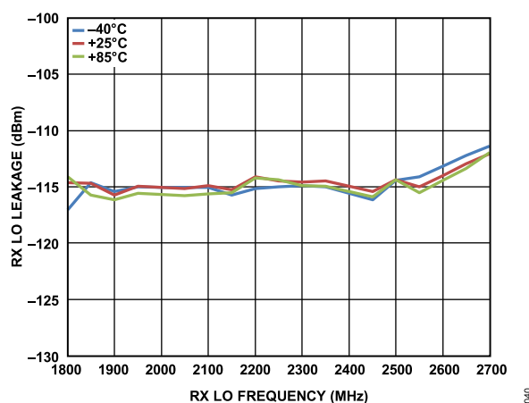
Figure 40. RX Local Oscillator (LO) Leakage vs. RX LO Frequency
