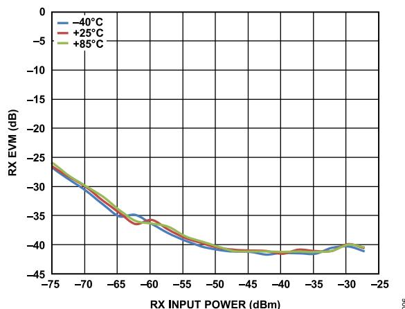
Figure 6. RX EVM vs. RX Input Power, 64 QAM LTE 10 MHz Mode, 19.2 MHz REF_CLK
