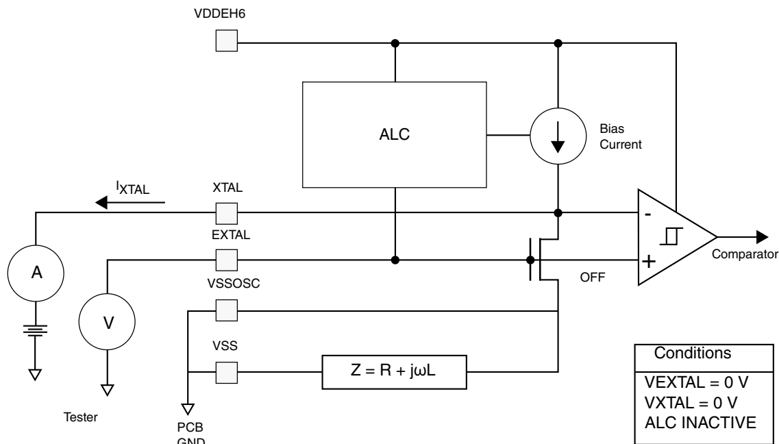
Figure 7. Test circuit
