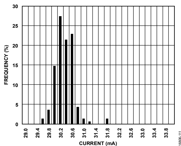
Figure 22. Operating Mode Current Distribution at 3.3 V Supply
