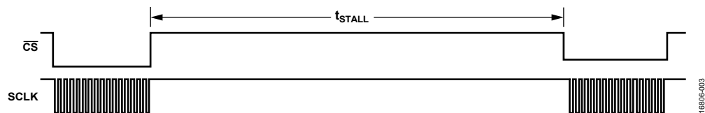
Figure 3. Stall Time (Does Not Apply to RTS Mode)
