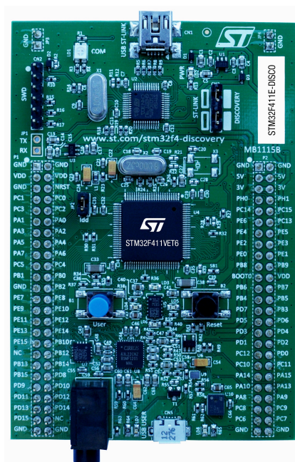
32F411EDISCOVERY top view. Picture is not contractual.
