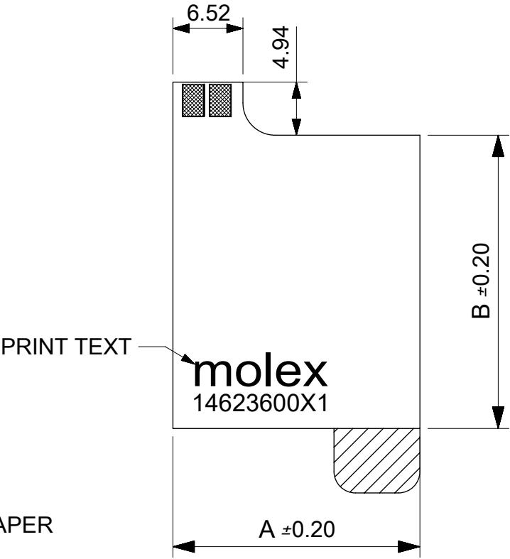
NFC ANTENNA WITHOUT FERRITE THICKNESS 0.17+/-0.05MM
