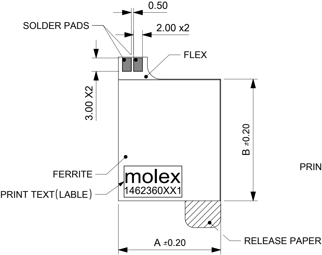
NFC ANTENNA WITH FERRITE THICKNESS 0.27+/-0.07MM
