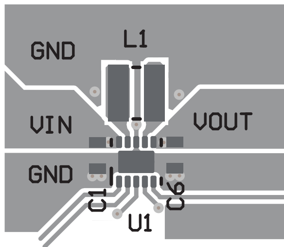
Figure 10-1. PCB Layout Example
