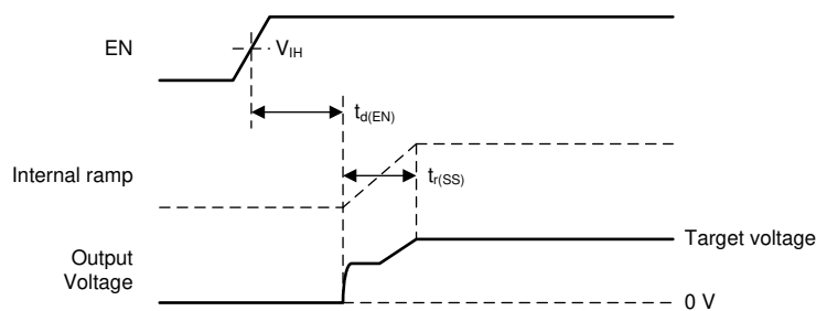
Figure 7-6. Start-Up Behavior
