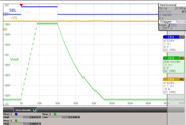
Figure 8-40. Short Circuit Behavior
