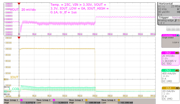
Figure 8-22. Load Transient, 100 mA Step
