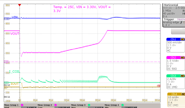
Figure 8-38. Start-up with 100-mA ICL
