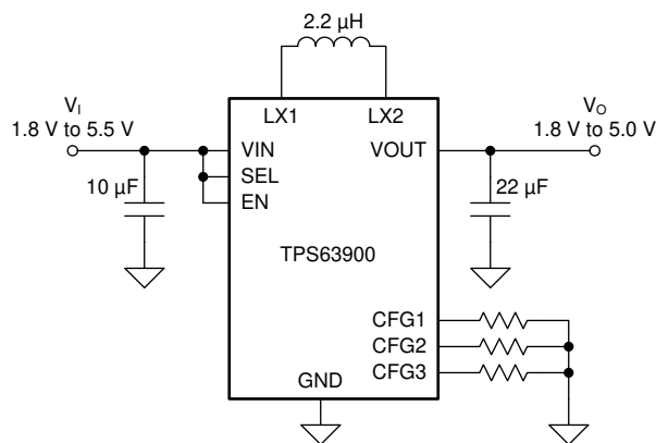
Simplified Schematic
