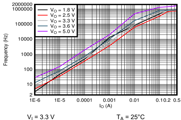
Figure 8-3. Typical Burst Switching Frequency versus Output Current
