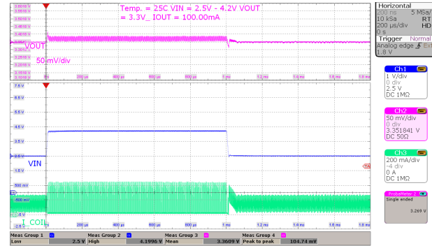
Figure 8-21. Line Transient, High Load
