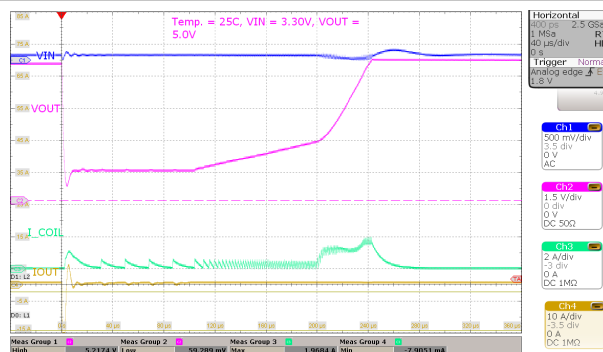
Figure 8-39. Short Circuit Behavior
