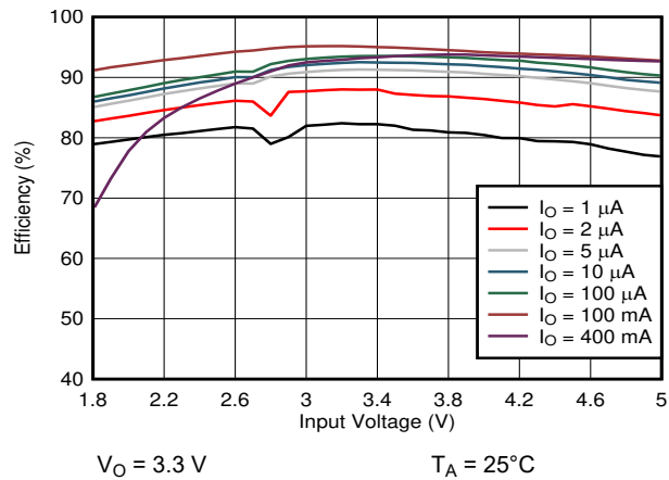
Figure 8-9. Efficiency versus Input Voltage
