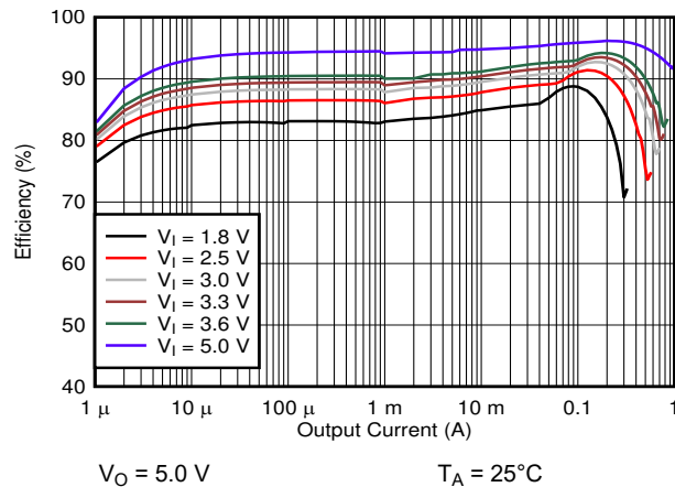
Figure 8-8. Efficiency versus Output Current
