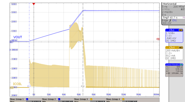
Figure 8-31. Start-up Behavior from Rising Enable
