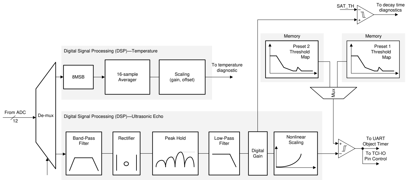
Figure 7-5. DSP Data-Path
