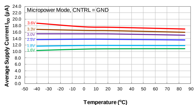
Average Supply Current (CNTRL = GND) vs Temperature
