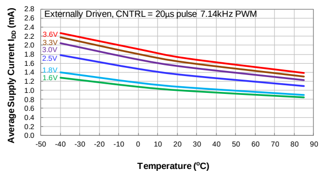
Average Supply Current (CNTRL = PWM) vs Temperature
