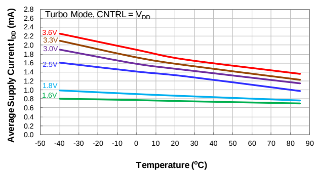
Average Supply Current (CNTRL = V_{DD} ) vs Temperature
