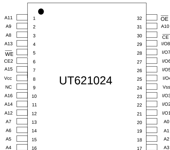
PDIP / SOP
