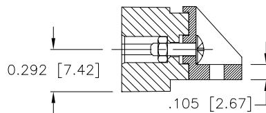
SECTION U-U
