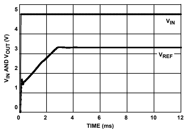
FIGURE 97. TURN-ON TIME ( +25^\circ C )
