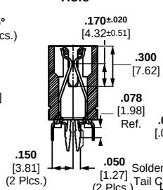
Section L-L
