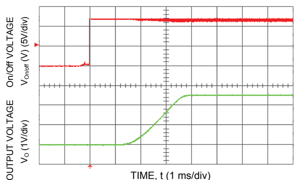
Figure 15. Typical Start-Up Using Remote On/Off with Low-ESR external capacitors ( C_o = 5000\text{ }\mu\text{F} ) ( V_{in} = 12.0\text{ Vdc} , V_o = 5.0\text{ Vdc} , I_o = 10.0\text{ A} , C_o = 1050\text{ }\mu\text{F} ).
