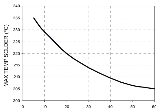
Figure 35. Time Limit Curve Above 205°C for Tin/Lead (Sn/Pb) process.
