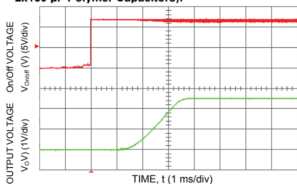
Figure 14. Typical Start-Up Using Remote On/Off ( V_{in} = 12.0\text{ Vdc} , V_o = 5.0\text{ Vdc} , I_o = 10.0\text{ A} ).
