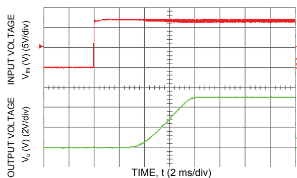
Figure 16. Typical Start-Up with application of V_{in} with low-ESR polymer capacitors at the output ( 7 \times 150\text{ }\mu\text{F} ) ( V_{in} = 12\text{ Vdc} , V_o = 5.0\text{ Vdc} , I_o = 10\text{ A} , C_o = 1050\text{ }\mu\text{F} ).
