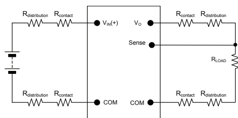
Figure 29. Remote sense circuit configuration
