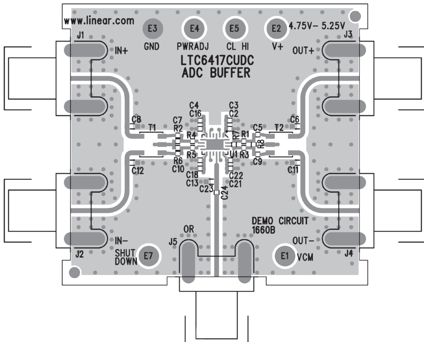
Figure 16. Demo Board DC1660B Layout
