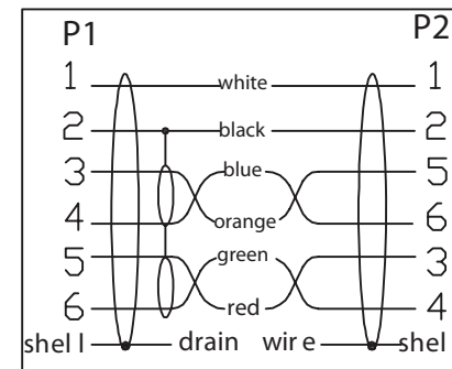
Wire Assignments
