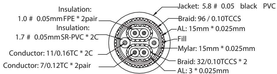
X-X Cross - Section
