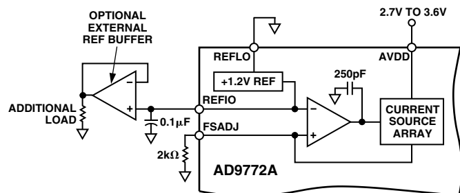
Figure 15. Internal Reference Configuration
