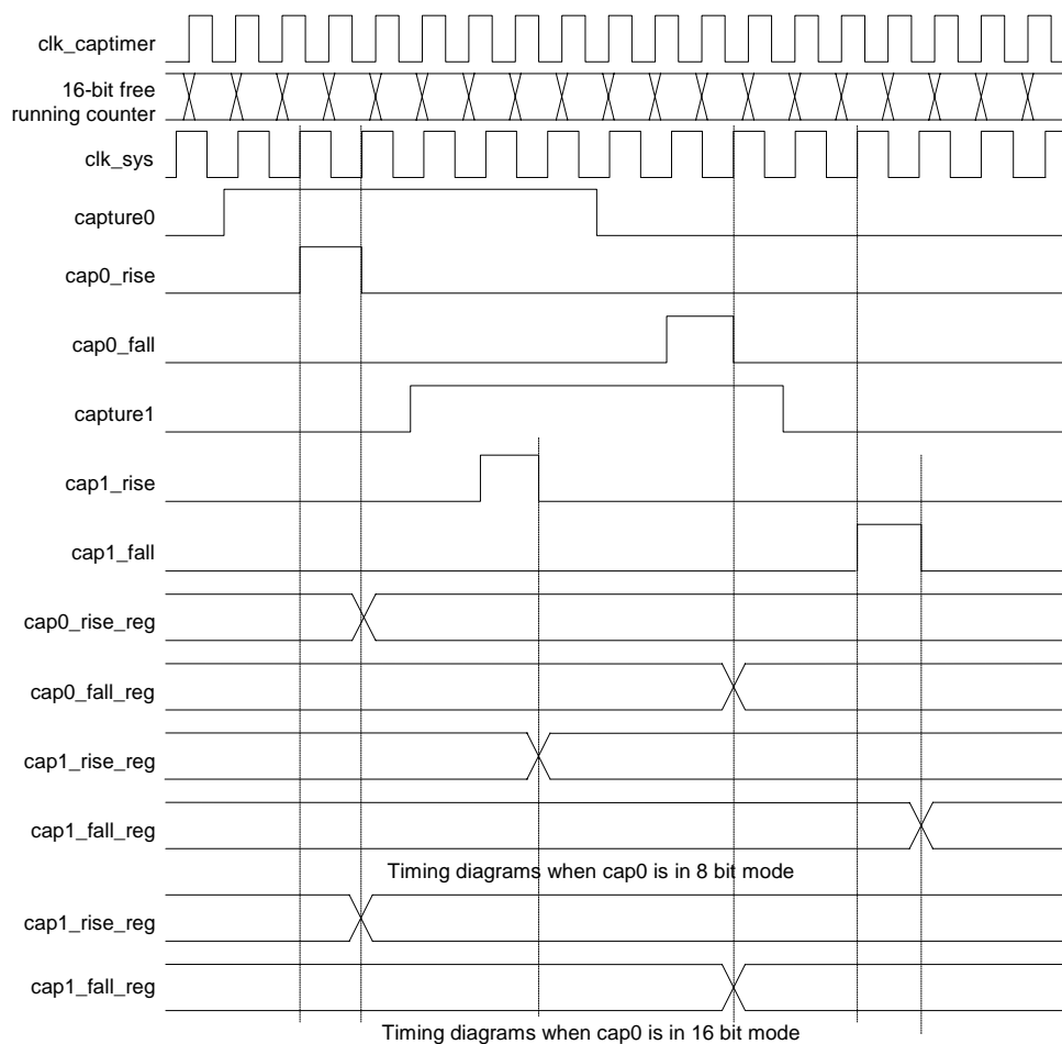
Figure 14. Timer Functional Timing Diagram
