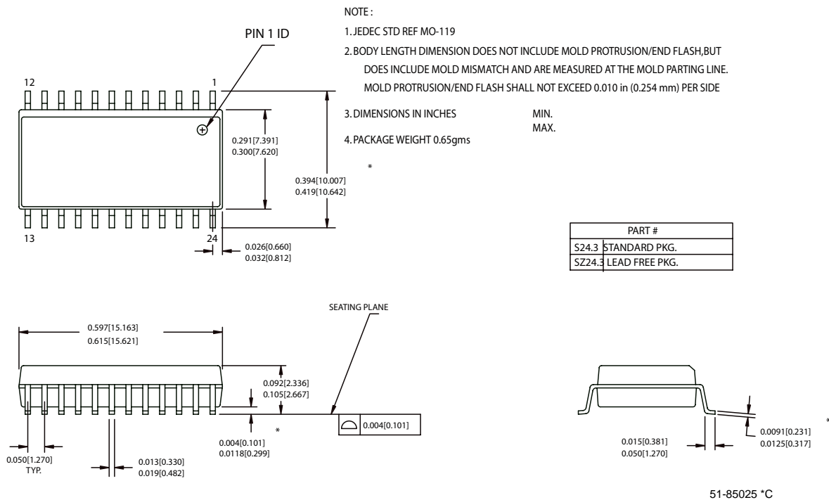
Figure 24. 24-Lead (300-Mil) SOIC S13
