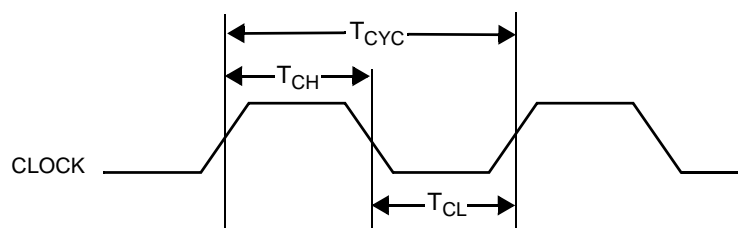
Figure 19. GPIO Timing Diagram
